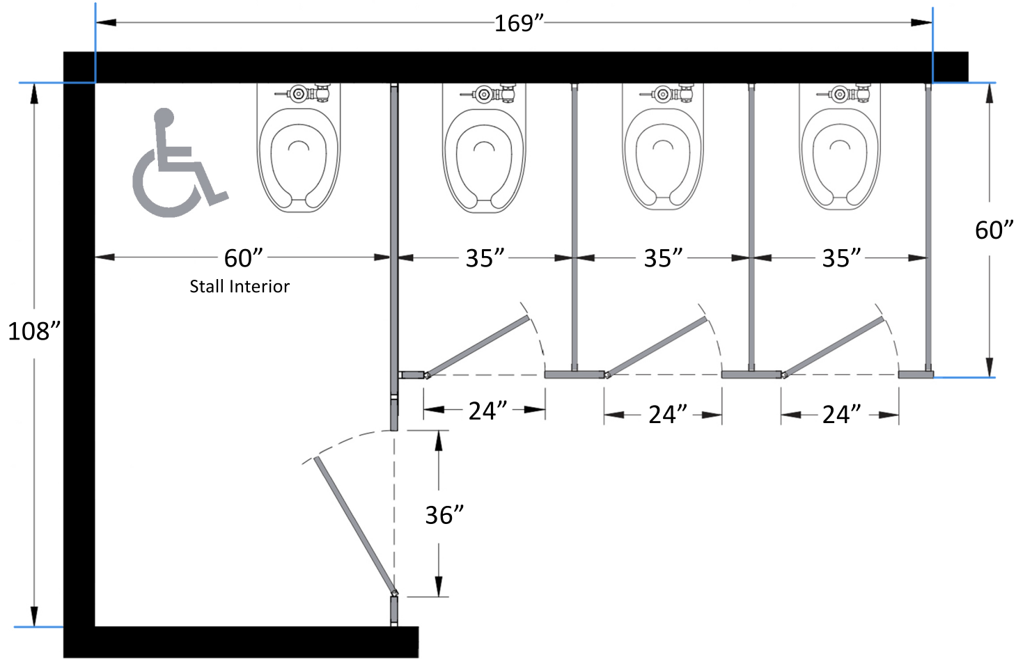
Bathroom Partitions - 4 Stall Alcove Left Hand ADA SKU: ALIC4LADA Standard Dimensions
